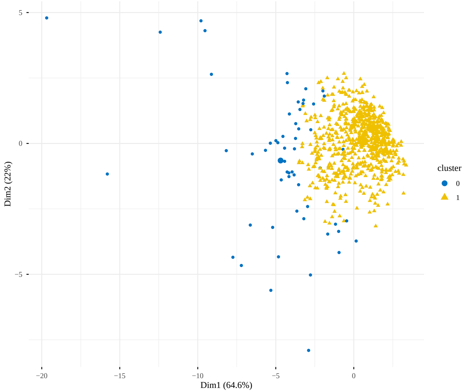
DBSCAN Clustering (eps = 1, minPts = 14)
